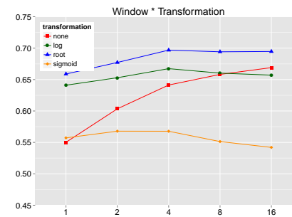
Rubenstein & Goodenough
