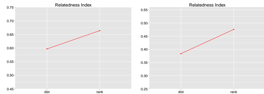
Rubenstein & Goodenough
