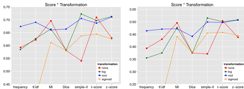
Rubenstein & Goodenough
